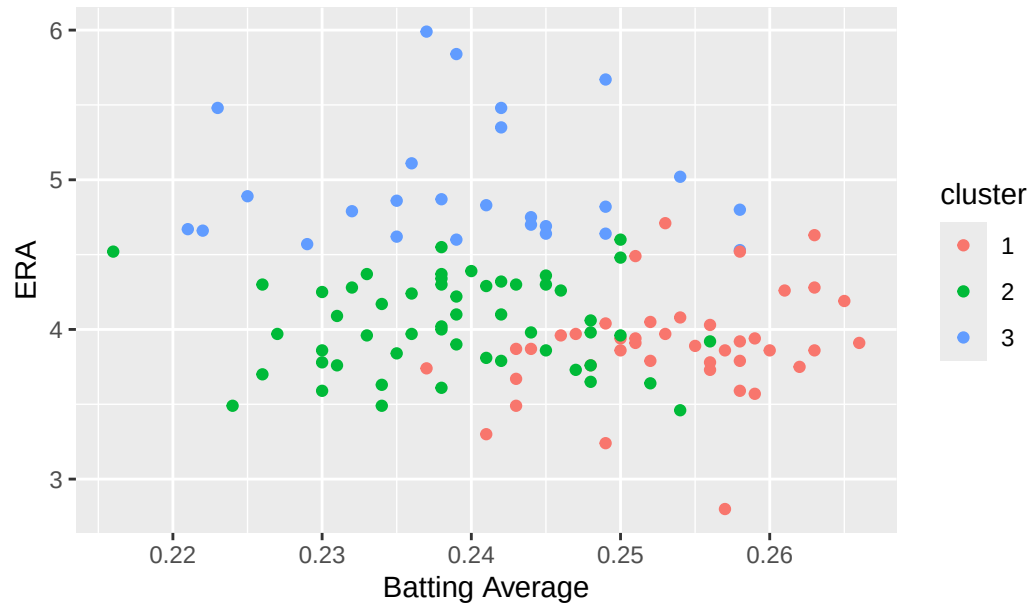
K-means Clustering of MLB Teams (2021+) (k=3)
